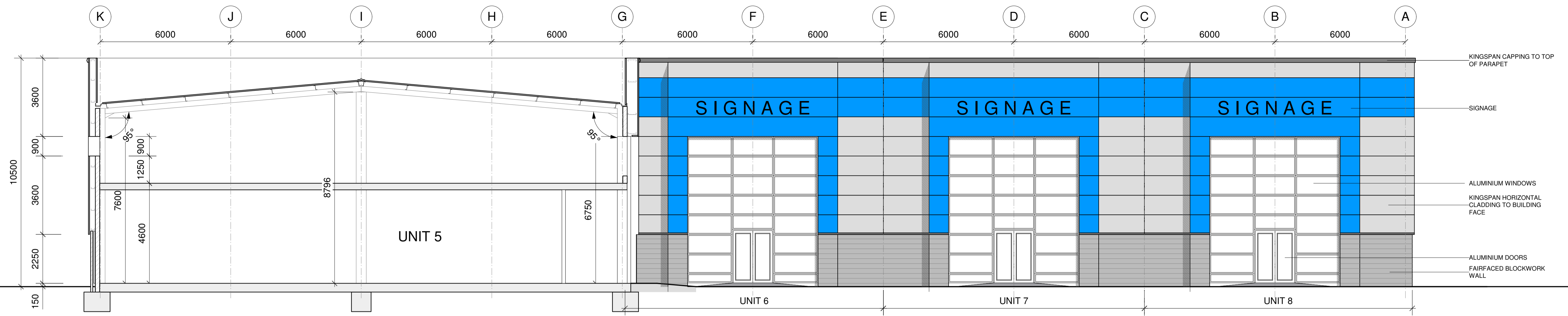
SECTION / ELEVATION
