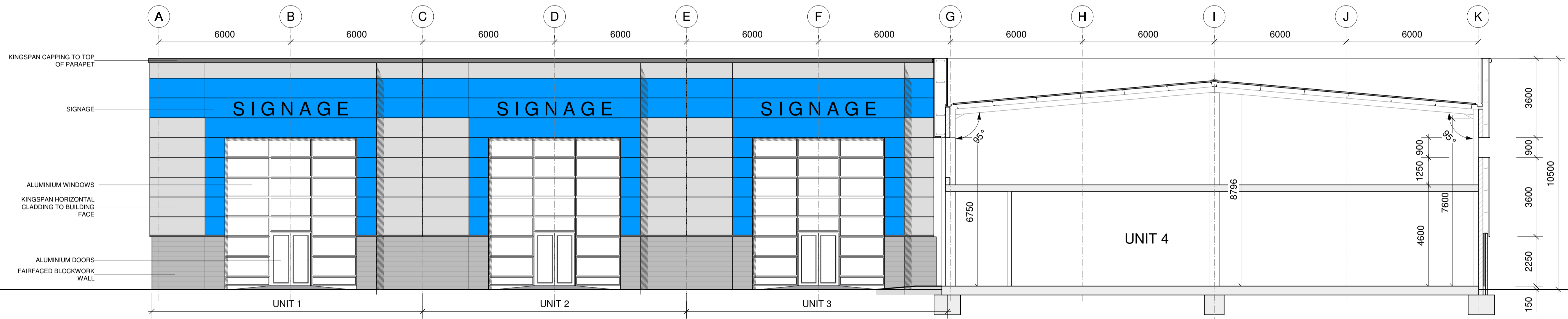
ELEVATION / SECTION
